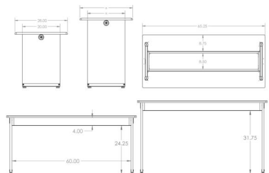
MOD2965-H + MOD3765-Q Drawing
